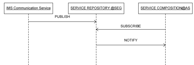
Figure 2: Sequence chart in service publishing and service discovery
